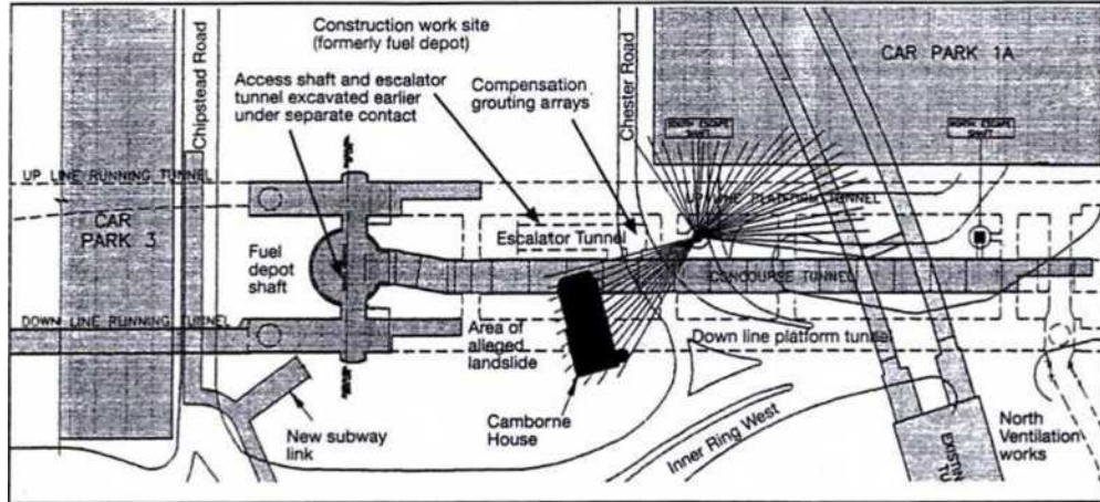
3 Plan of the excavation works completed at the time of the collapse of the Central Terminal Area
